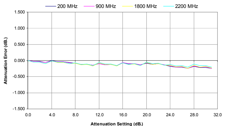
Figure 14. 1dB Attenuation Error vs. Frequency
