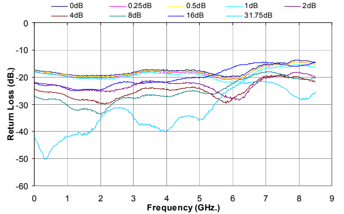
Figure 18. Output Return Loss vs. Attenuation T = +25C
