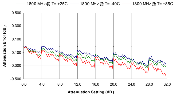
Figure 24. Attenuation Error vs. Attenuation Setting @ 1800 MHz
