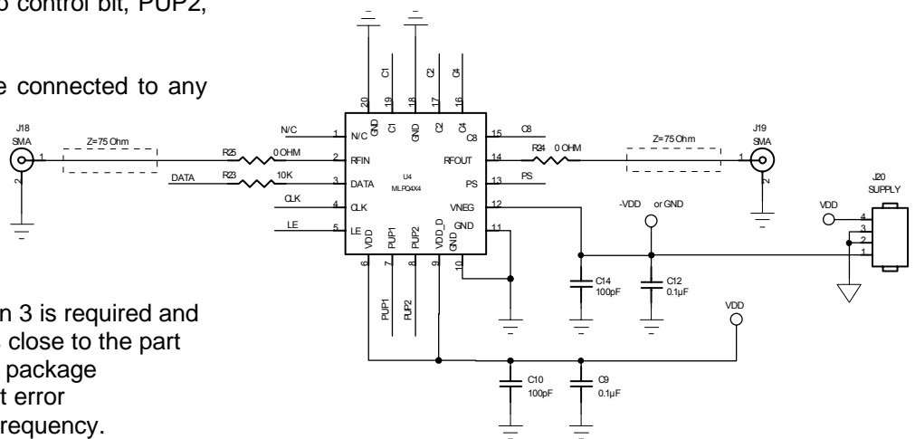
Figure 5. Evaluation Board Schematic
