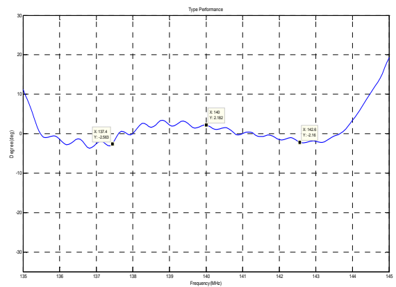
Phase Linearity(f0±2.6MHz)
