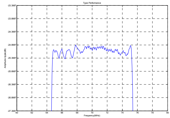
Passband Respond
