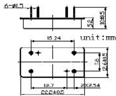
Package Outline
