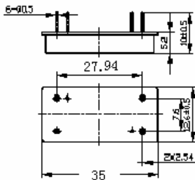
Package Outline
