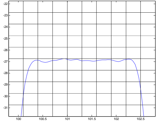
Phase Linearity( f_0 \pm 1.1 MHz)
