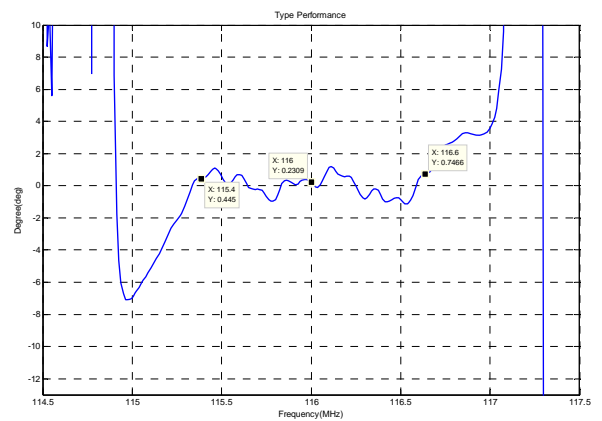
Phase Linearity(f0±0.6MHz)
