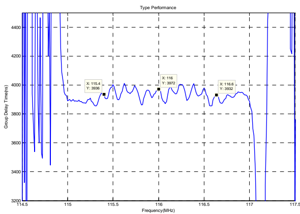
Group Delay Variation(f0±0.6MHz)
