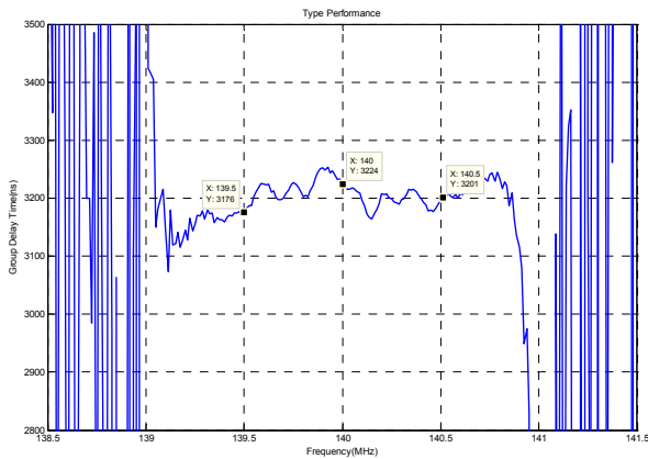
Group Delay Variation(f0±0.5MHz)
