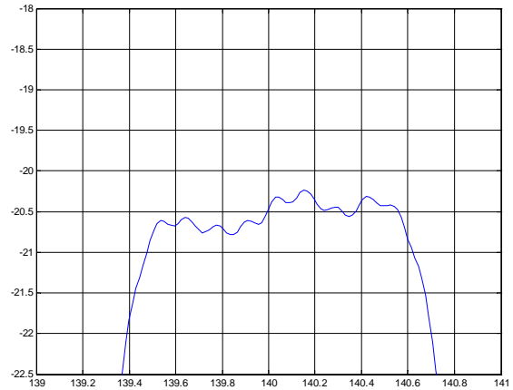
Phase Linearity( f_0 \pm 0.6 MHz)
