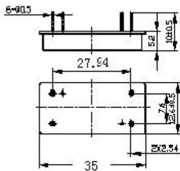
Package Outline
