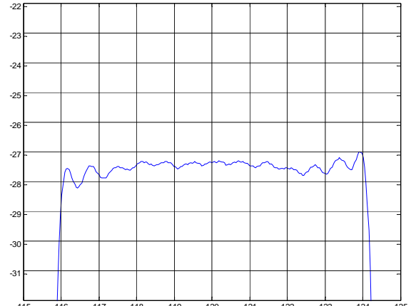
Phase Linearity( f_0 \pm 4\text{MHz} )
