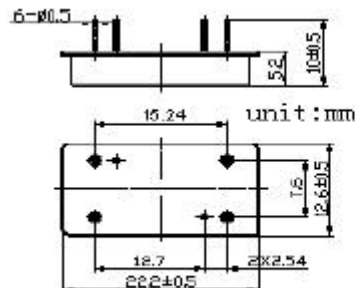
Package Outline
