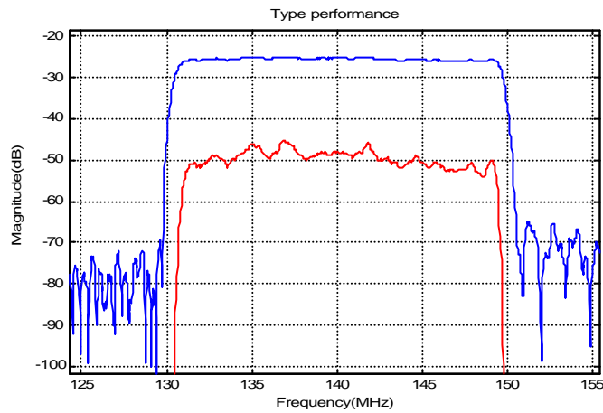
SP140B19 SAW Filter Typical Performance
