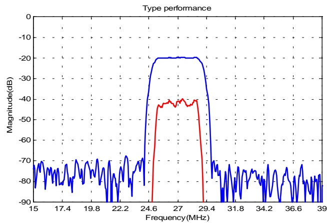
SP27-3.5 SAW Filter Typical Performance
